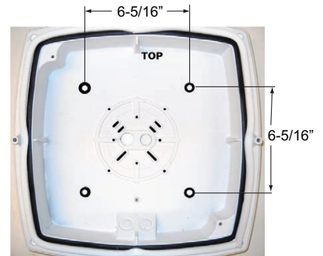
Linz Mounting Dimensions
