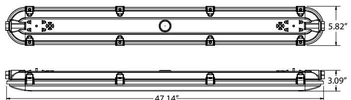
Low Profile Lens Dimensions
